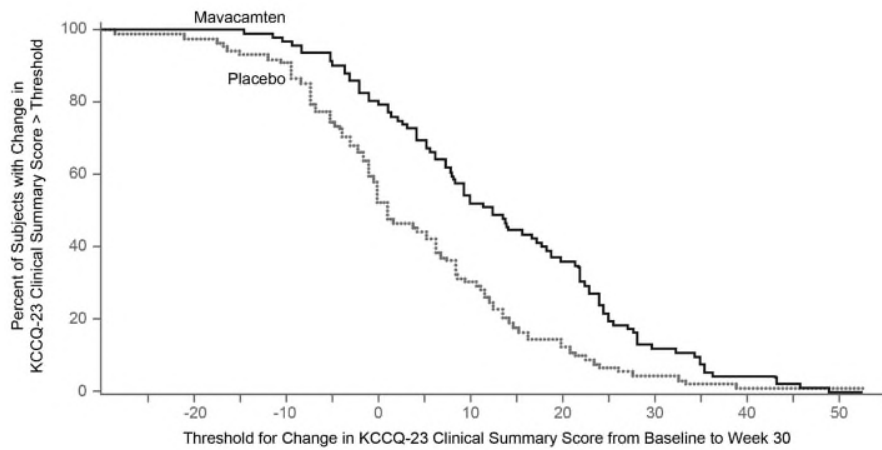
Figure 4: KCCQ-23 CSS: Cumulative Distribution of Change from Baseline to Week 30
